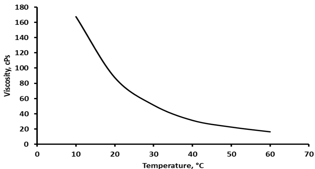
Viscosity as a Function of Temperature
